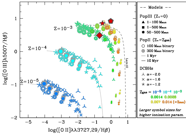
Figure 4. [\text{O III}]/\text{H}\beta vs [\text{O II}]/\text{H}\beta diagram illustrating the photoionization models for low metallicity PopII, PopIII and AGNs from Nakajima & Maiolino 2022. Different symbols mark different population of objects (as explained in the legend), while different colours belong to different values of the gas-phase metallicity. The line ratios observed in our z \sim 8 galaxies are marked with red symbols.
