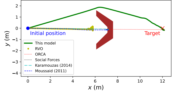
FIG. S1. Local navigation of one agent around a non-convex obstacle towards a predefined target, simulated with ANDA ('this model') and with alternative agent-based models: RVO [67], ORCA [68], social force model [16], Karamouzas et al.'s TTC-based model [21], Moussaid et al.'s heuristic model [22]. These other models were simulated using their implementation in the UMANS software with their native parameters in this software.
