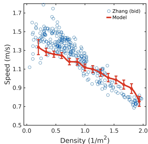
FIG. 7. Variation of the average pedestrian speed with the mean density in a bidirectional corridor flow.
