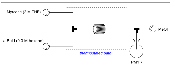
Fig. 2. Flow polymerization of myrcene.
