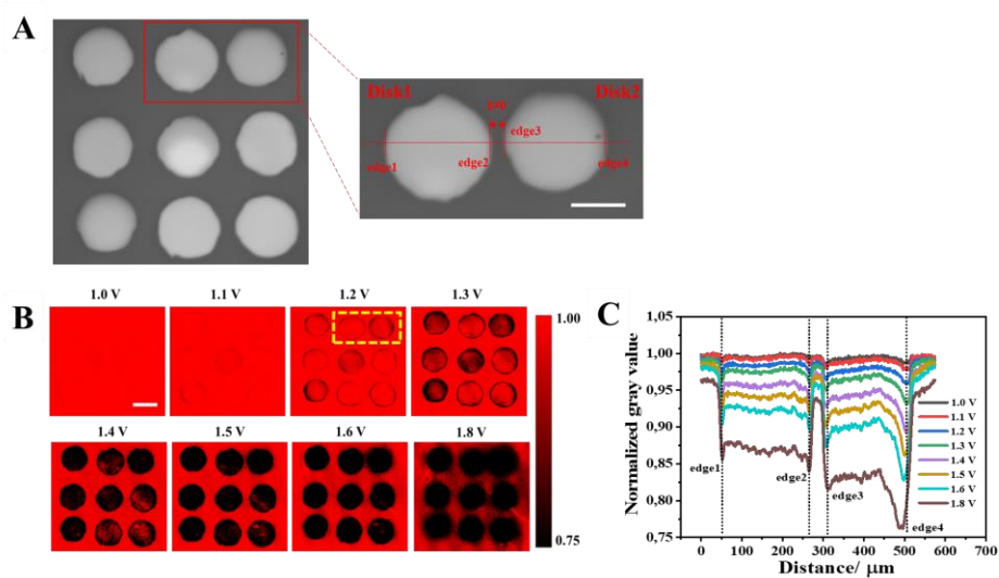
Fig. 7. (A) Optical micrograph of Au disks sputtered on ITO. Scale bar (white): 100 \mu\text{m} . (B) The images for optical change of CE with increasing voltage at the WE made of sputtered Au array on ITO (Scan rate: 0.05 V/s). Scale bar (white): 200 \mu\text{m} . (C) The variation of normalized gray value of the two micro-disks on CE (the yellow dotted frame in Fig. 7B) with increasing the voltage. The edges (1–4) correspond to the edges of the two micro-Au disk on the WE in Fig. 7A, respectively.
