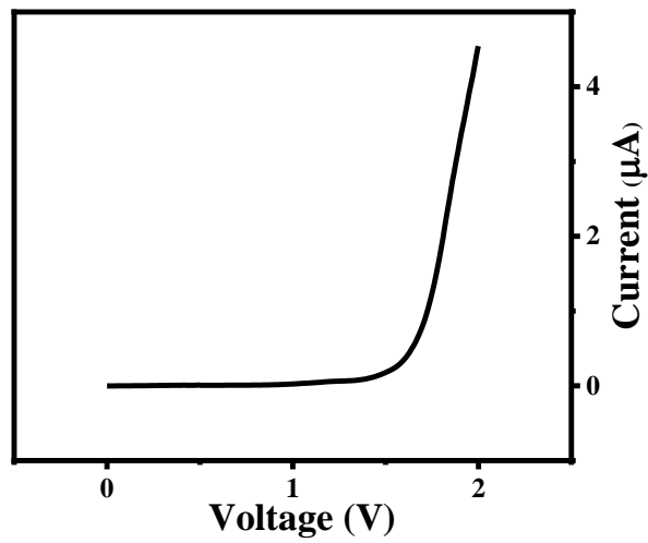
Fig. S2. Current vs. voltage curves of electrochemical cell consisting of gold microelectrode array as WE, \text{WO}_3/\text{ITO} as CE, 10 \mu\text{m} PTFE as spacer. Scan rate: 0.05 V/s.
