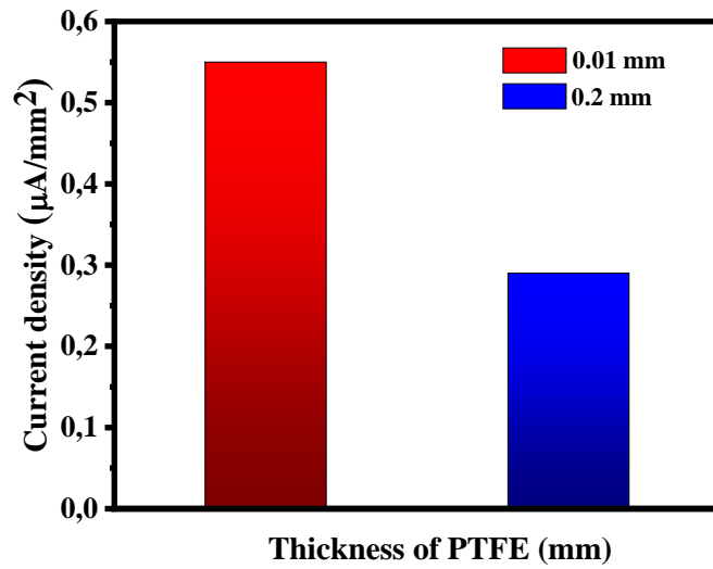
Fig. S1. The current density of electrochromic device for two different thicknesses of the PTFE spacer: 0.2 mm and 0.01 mm. Voltage: 1.5 V; Time: 5 s.
