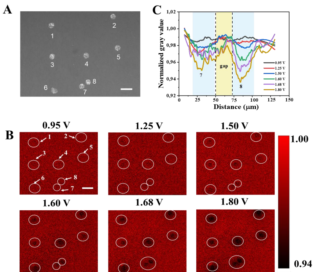
Fig. 6. (A) Optical micrograph of Au microelectrode array. The scale bar (white): 50 \mu\text{m} . (B) The images for optical change of CE at different voltage. Scale bar: 50 \mu\text{m} . (C) The variation of normalized gray value of the region 7, 8, and the gap on CE with increasing the voltage.
