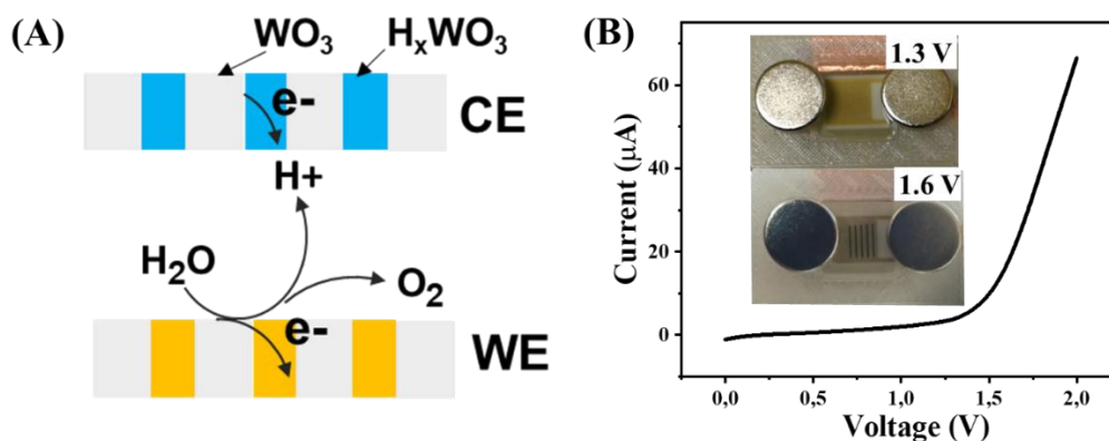
Fig. 2. (A) Schematic diagram of the reaction mechanism of a gold interdigitated WE array (yellow) and \text{WO}_3 film CE (where the localized oxidation is depicted in blue). (B)
