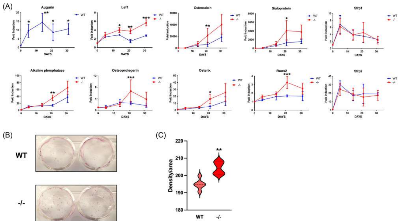
FIGURE 2 Accelerated osteogenic differentiation of Ecr4 -/- osteoblasts. (A) Osteoblast differentiation marker gene expression during the time course of osteogenic differentiation of osteoblasts isolated from wild-type (WT) (blue) and Ecr4 -/- (red) neonatal mice measured by real-time quantitative polymerase chain reaction (RT-qPCR). n = 3-5 . * p < .05 ; ** p < .01 ; *** p < .001 , REST analysis. (B) Alizarin Red staining of WT and Ecr4 -/- osteoblasts at day 21 of differentiation. The staining adjacent to the side of the well is artifactual. (C) Alizarin Red staining quantification at day 31 of differentiation in WT and Ecr4 -/- osteoblasts. Results are expressed in optical density units normalized by the area of osteoblast culture. n = 3 , ** p < .01 , Mann-Whitney test
