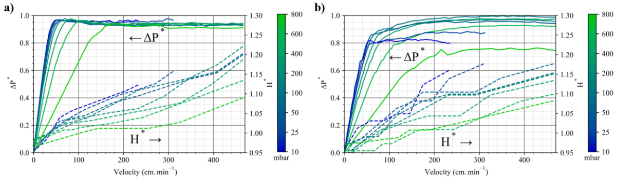
Figure 6 : Normalized pressure drop ( \Delta P^* in solid lines) and normalized expansion ( H^* in dashed lines) of a) the pure SiC powder bed and b) 30f/70p mixture, as a function of pressure and gas velocity.
