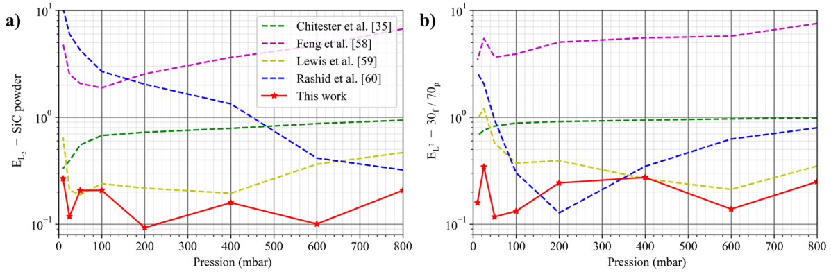
Figure 10 : Weighted squared errors as a function of pressure for a) the pure SiC powder and b) the 30p/70p mixture.
