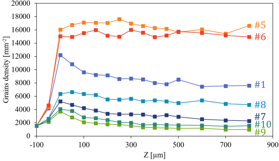
Figure 12: Grains density of REV simulations versus height in the multidirectional scanning strategies (#5, #7-#10) S_L^{XY} and (#6) S_L^{67} compared to the monodirectional scanning strategy S_L^X (#1) (Tab. 3).
