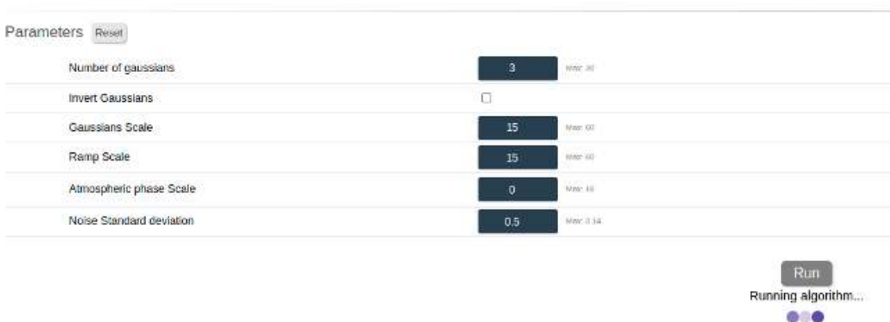
Figure 3: Interface of the demo. Each input in a blue box is of numeric type. The maximum value is shown on the right. The number of Gaussians should be an integer, while others can be floating-point scalars. Invert Gaussians is a Boolean represented by a checkbox on the interface. The default values that are shown yield images similar to the training data.
