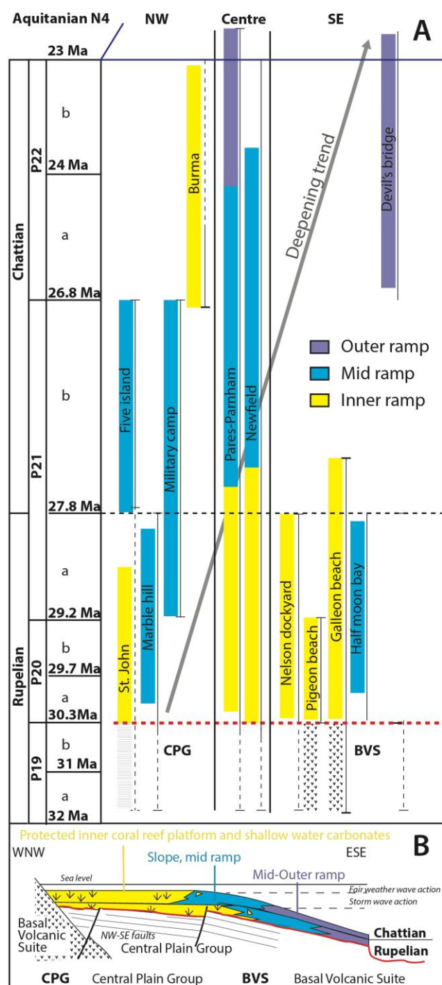
909 Figure 10. A: Depositional settings of the Antigua Fm. with ages from the 910 biostratigraphic investigations (Appendix 1 and 2); B: Synthetic sedimentary 911 organization during the late Rupelian and the Chattian. The Antigua Fm. was 912 deposited on a northeastward, low-angle dipping ramp. The underlying Central Plain 913 Group was previously faulted and tilted by NW-SE normal faults. For sites location, 914 see Fig.3.
