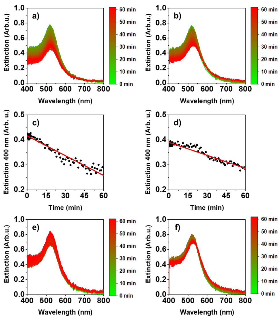
Figure S2: Time evolution of the ensemble extinction spectra when the ion concentration is 0.125 M, at 45 °C (a) and 55 °C (b). Decrease in extinction at 400 nm as a function of the elapsed time
