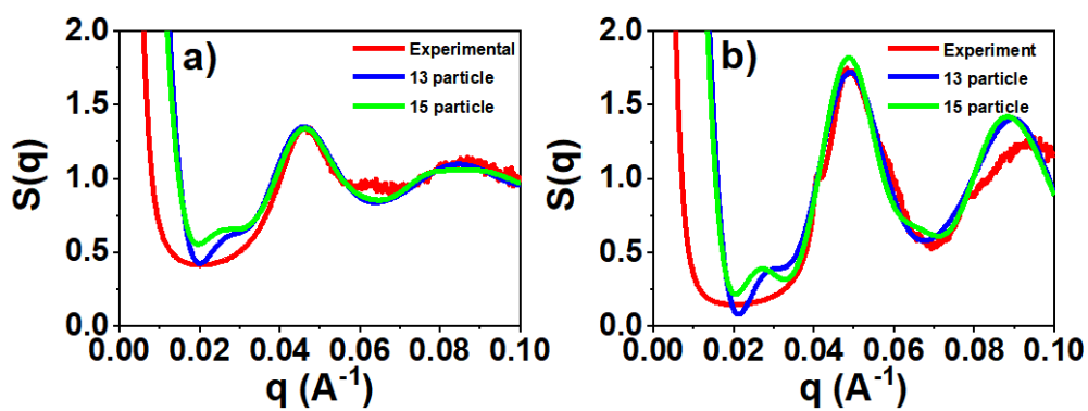
Figure S6: Experimental and calculated structure factors assuming 13 or 15 particles in the clusters for 0.125 M; 45^\circ\text{C} (a) and 0.25 M; 55^\circ\text{C} (b).
