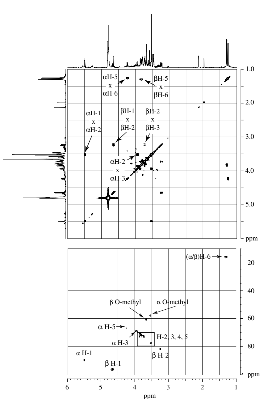
Fig. 4. ^1\text{H} NMR COSY (top) and HSQC spectra (bottom) of fraction \text{F}_3\text{C1} (2- O -methylfucose; XVII). The 1-D ^1\text{H} NMR spectrum of \text{F}_3\text{C1} is projected on the X- and Y-axes of the top panel for reference. Cross peaks in COSY spectrum are due to coupling between adjacent protons and are used to assign signals in the 1-D spectrum. ^1\text{H} NMR spectra assignments are then used to determine carbon chemical shifts in the HSQC spectrum (lower panel).
