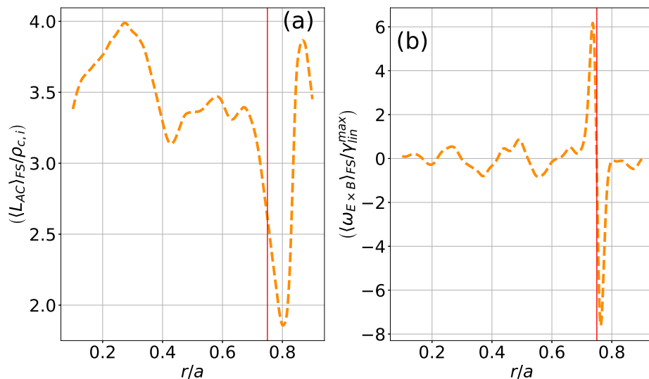
Figure 16: Flux surface and time average of the correlation length (a) and E \times B shearing rate (b) as a function of radius for the step gradient case. The red vertical line indicates the step gradient location.
