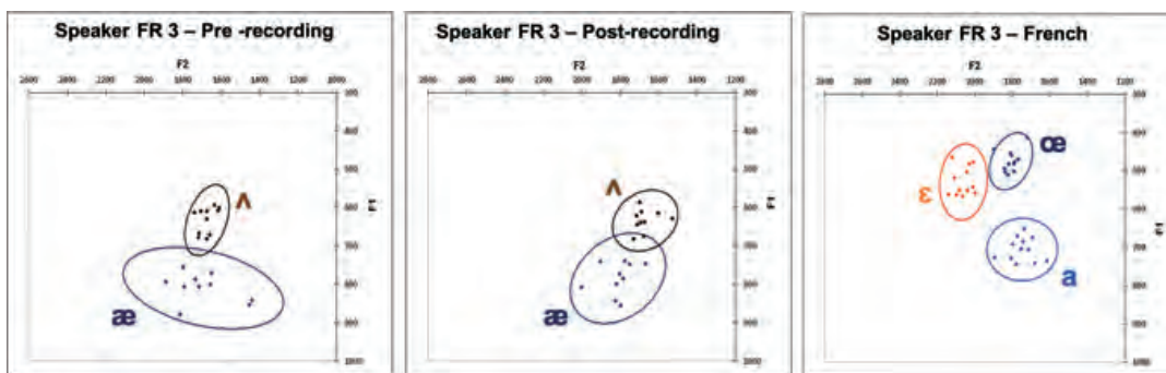
Fig. 5: F1/F2 ellipse plot of /æ/ and /ʌ/ as produced by speaker FR3 in the pre-training (left) and post-training (middle) condition, together with the control productions of French /ɛ, a, œ/ (right).
