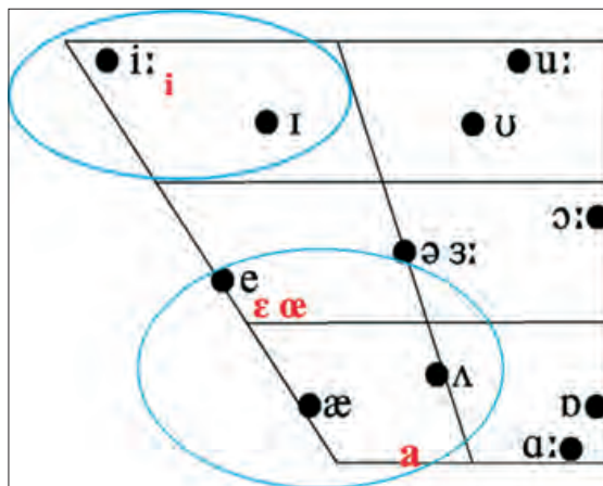
Fig. 2: The IPA vowel diagram for Standard Southern British English (in black) and the four French vowels (in red) used for comparison. The target vowels are indicated by the ellipses.
