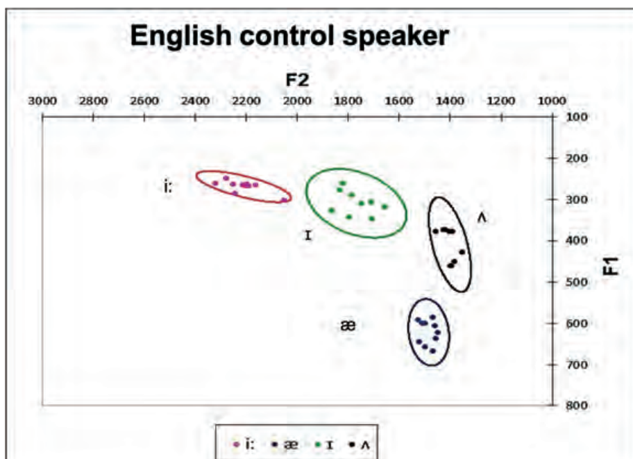
Fig. 3: F1/F2 ellipse plot of English target vowels as produced by the British control speaker.
