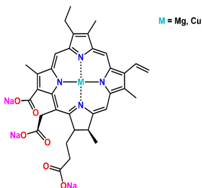
Fig. 1. Structure of the sodium magnesium chlorophyllin ( C_{34}H_{31}MgN_4Na_3O_6 , M=684.92 g.mol -1 ) or sodium copper chlorophyllin ( C_{34}H_{31}CuN_4Na_3O_6 , M=724.15 g.mol -1 ).
