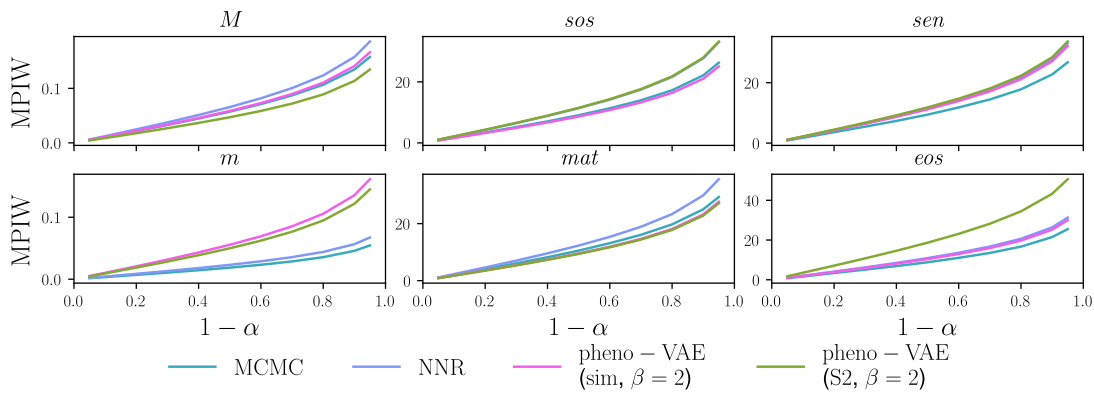
Fig. 19. MPIW vs 1 - \alpha for MCMC, Neural Network regression and pheno-VAE (with \beta = 2 , trained on the S2 or simulated data-set). prediction interval sizes are similar for all methods, except for m , where prediction intervals are larger for pheno-VAE, and for the eos of pheno-VAE trained on the S2 data-set, that also has larger prediction intervals.
