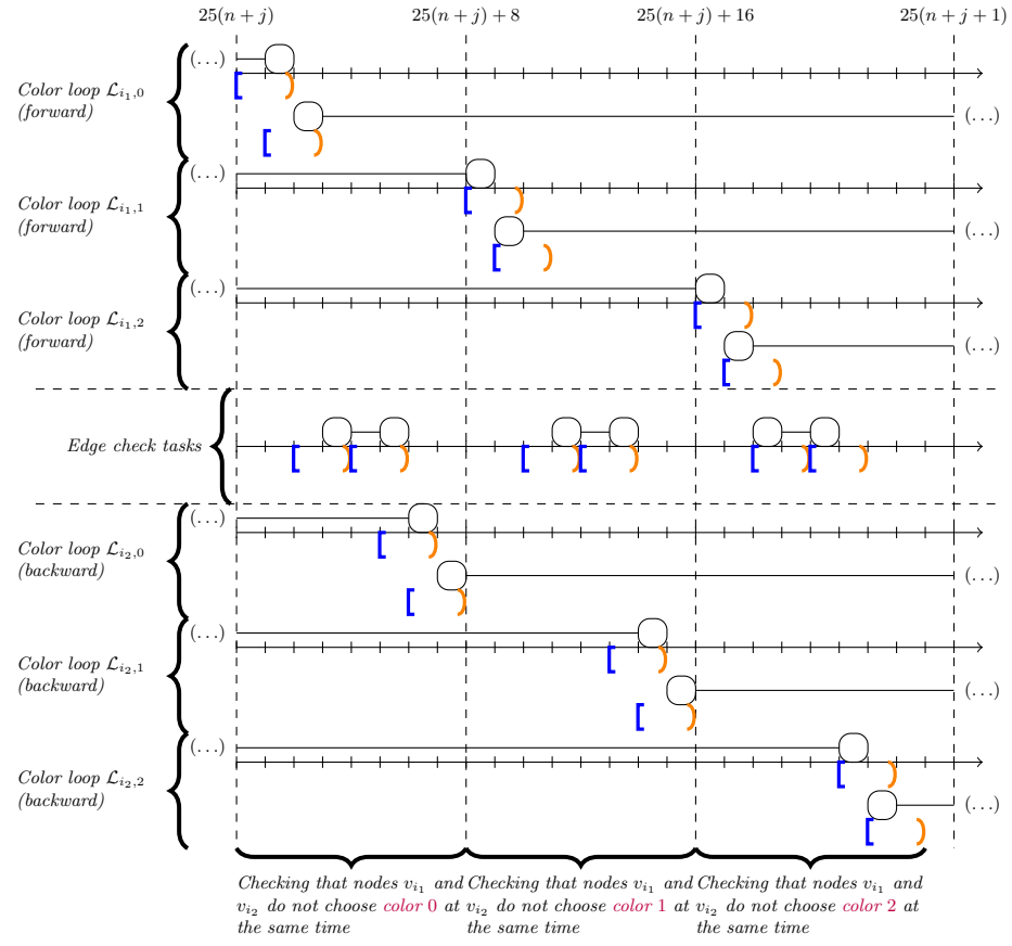
Fig. 3. The edge check segment corresponding to edge e_j = \{v_{i_1}, v_{i_2}\} with i_1 < i_2 in the reduction with minimum delays. Here color loops \mathcal{L}_{i_1,0} and \mathcal{L}_{i_2,2} are ON and the other four are OFF.
