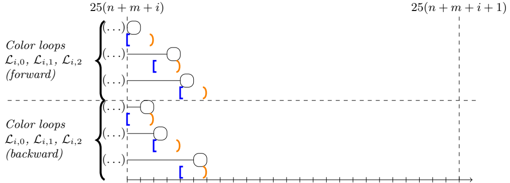
Fig. 7. The closing segment corresponding to node v_i in the reduction with maximum delays. Here color loop \mathcal{L}_{i,1} is OFF and the other two are ON.
