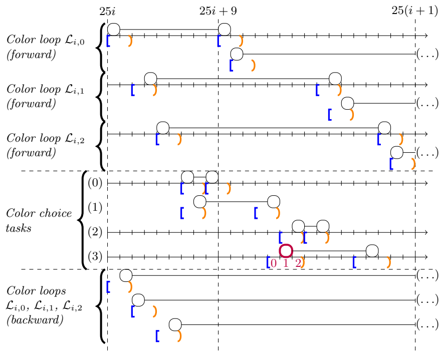
Fig. 2. The color choice segment corresponding to node v_i in the reduction with minimum delays. Color loop \mathcal{L}_{i,1} is ON and the other two are OFF.
