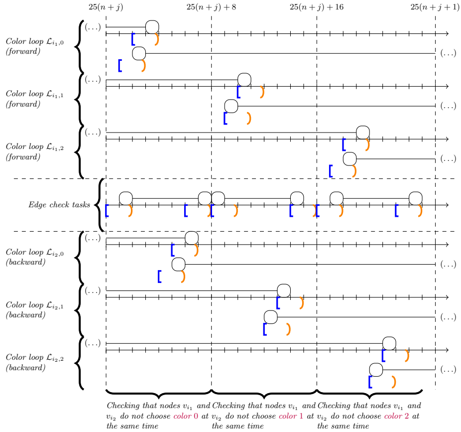
Fig. 6. The edge check segment corresponding to edge e_j = \{v_{i_1}, v_{i_2}\} with i_1 < i_2 in the reduction with maximum delays. Here color loops \mathcal{L}_{i_1,1} and \mathcal{L}_{i_2,0} are ON and the other four are OFF.
