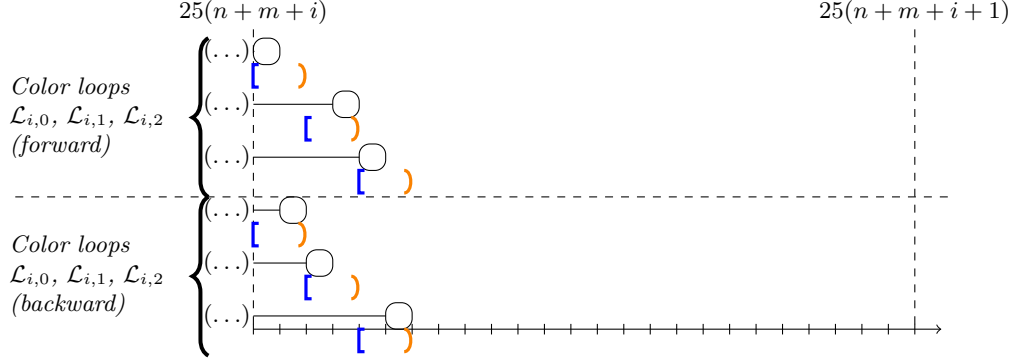
Fig. 4. The closing segment corresponding to node v_i in the reduction with minimum delays. Here color loop \mathcal{L}_{i,1} is ON and the other two are OFF.
