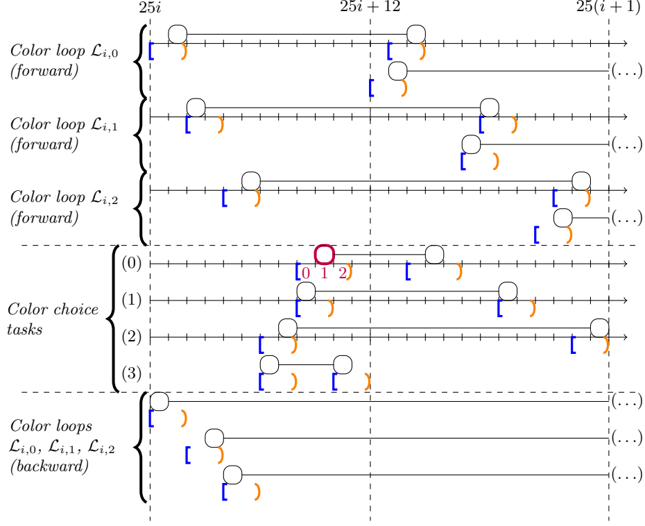
Fig. 5. The color choice segment corresponding to node v_i in the reduction with maximum delays. Color loop \mathcal{L}_{i,1} is ON and the other two are OFF.
