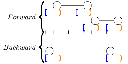
Fig. 1. A loop of properly coupled tasks for minimum delays.
