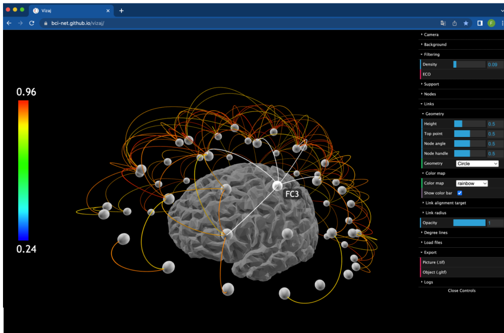
Fig 2. Screenshot of the Vizaj 's graphical user interface (GUI). Spatial networks are built in a 3D scene. The network can be zoomed and rotated via the cursor input. When the cursor hit a node, its connections and label are dynamically highlighted. On the right, all the controlling parameters are listed and accessible to the user.
