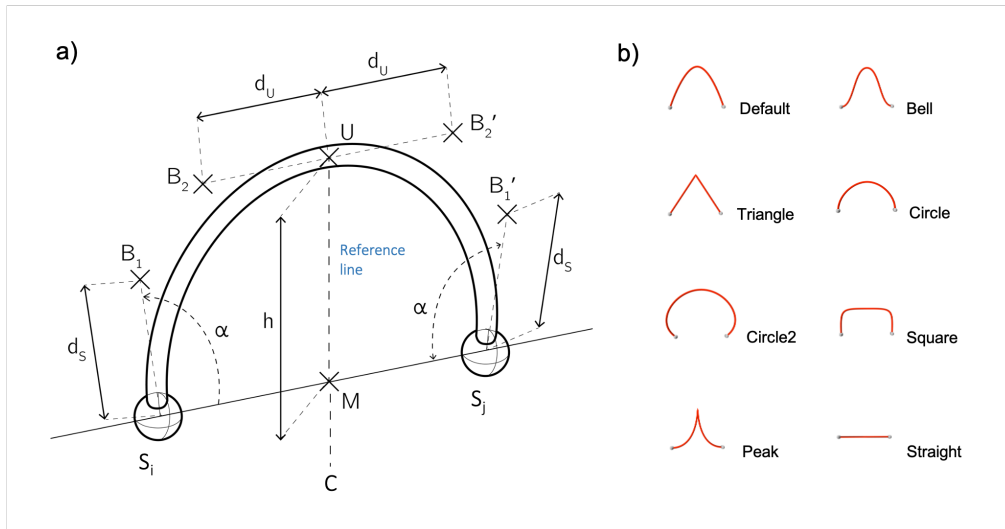
Fig 1. Geometric principles for shaping links. a) Schematic illustration of the parameters controlling the shape of the link between two nodes S_i and S_j . The reference point M lies on the geodesic distance d_{ij} between the nodes. Bezier boundary points are referred as to B and can be moved by modulating four quantities, ie h , d_U , \alpha and d_S . Note that the angles \widehat{B_2UM} and \widehat{B_2'UM} are always square and not customizable for the sake of simplicity. b) Typical configurations that can be obtained with different combinations of the controlling parameters a_1, a_2, a_3, a_4 in the GUI. Default (0.75, 0.5, 0.38, 0), Bell (0.75, 0.5, 0, 0.5), Triangle (0.75, 0, 0, 0), Circle (0.5, 0.5, 0.5, 0.5), Circle2 (0.9, 1, 0.8, 1), Square (0.5, 1, 0.5, 1), Peak (0.75, 0, 0, 1), Straight (0, 0, 0, 0).
