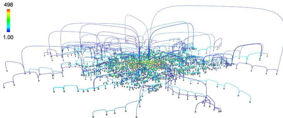
Fig 4. Paris public transports. Nodes are stops and links is travel connections. Mixed modes of travel are included (tram, rail, metro and bus). The color of the links indicates the number of vehicles that used that connection on a Monday. Only the connections covering a physical distance above 500 meters are displayed for the sake of simplicity. Data available from [13]. The network visualization has been generated with Vizaj using a Square shape for the links.
