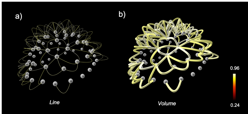
Fig 9. Graphical implementation of the links a) Line option: links are made of single pixels. b) Volume option: links are made of multiple adjacent cylinders along the path between the two connected nodes. This synthetic network has been visualized with Vizaj using a Default shape for the links.
