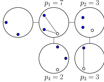
(d) Step 3, p_1 has decreased by 1. k = 13 .
