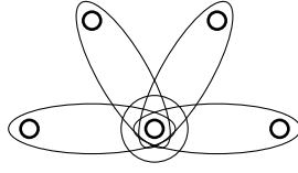
Figure 2: A hypergraph satisfying Ls(H) = \lfloor \frac{\Delta(H) + 1}{2} \rfloor in Maker-Maker convention
