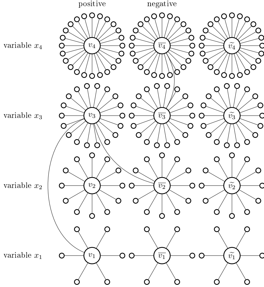
Figure 4: Reduction of \exists x_4 \forall x_3 \exists x_2 \forall x_1 (\neg x_2 \vee x_3) \wedge (x_1 \vee x_3) \wedge (\neg x_3 \vee \neg x_4)
