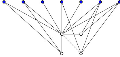
(e) Step 4, each vertex v_i has p_i blue neighbors.
