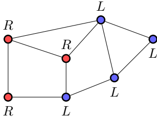
Figure 1: An endgame of INCIDENCE. In Maker-Maker convention the score of the position is 2 while it is 4 in Maker-Breaker convention.
