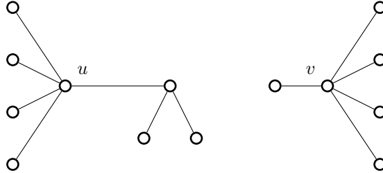
Figure 3: A graph G for which Ls(G) = 4 with unique optimal move u and Rs(G) = 2 with unique optimal move v .
