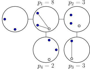
(c) Step 2, 16 edges removed, k = 30 - 16 = 14
