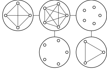
(a) A graph to kernelize. Set k = 30 .
