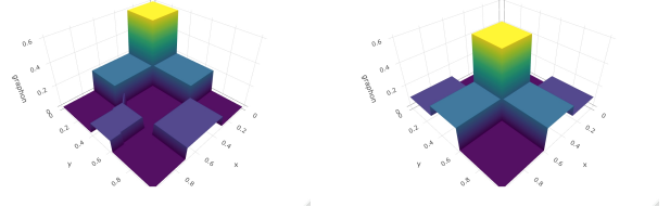
Fig. 2: Graphons of a SBM with two different orders of the block labels.
