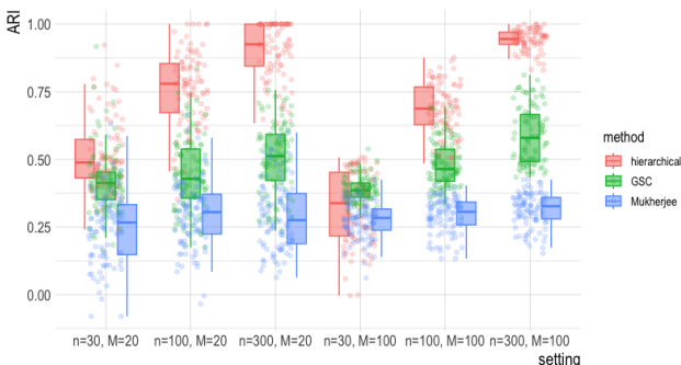
(b) ARI of network clusters
