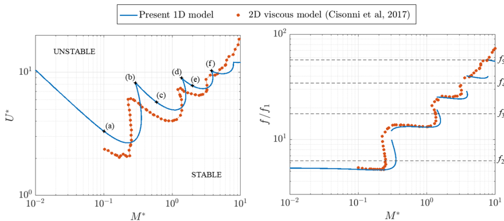
Figure 2 – Stability boundary in the (U^* - M^*) plane (left) and the corresponding frequencies (right) for a system with confinement H^* = 1/10 and Reynolds number Re = 100 . The 2-D model results were retrieved from those presented in [20].
