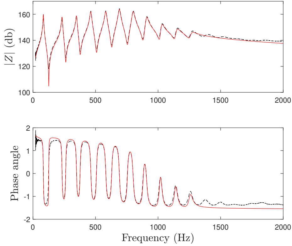
Figure 1: (Color online) Measured input impedance (dashed black) and reconstructed input impedance from 11 complex modes (red) for a Bb trumpet with open fingering.
