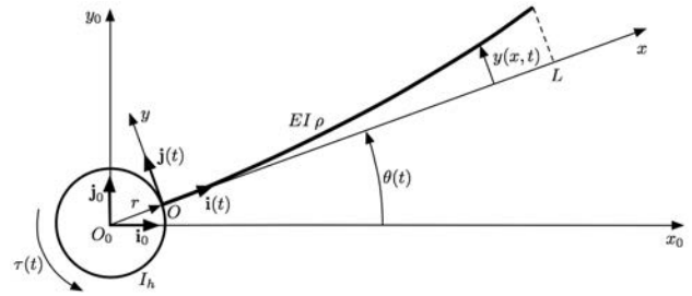
Fig. 1 Slewing flexible beam
