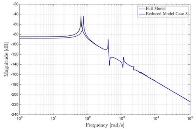
Fig. 15 Magnitude Bode diagrams of the full model TF and reduced model TF defined in Case 8 in Table 3
