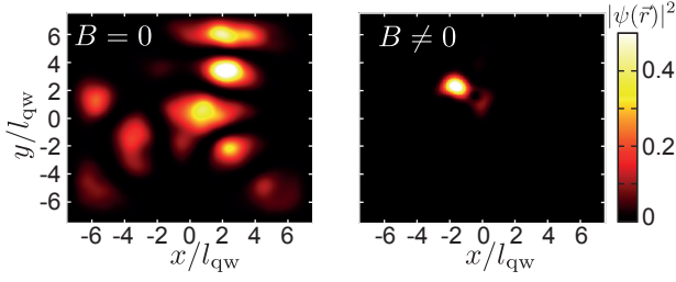
FIG. 7. Illustrative examples of the real-space wavefunction of a n = 1 subband eigenstate in the presence of disorder in the B = 0 (left) and B \neq 0 (right) cases.
