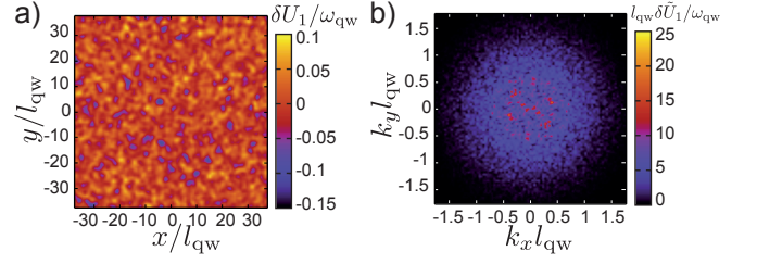
FIG. 2. a) Spatial profile of a single realisation of the disorder potential \delta U_n(\vec{r}) for the n = 1 subband. b) Fourier transform of the same disorder potential \delta \tilde{U}_n(\vec{k}) as a function of the wavenumber \vec{k} . Disorder parameters: \eta_{\text{dis}} \approx 0.06 , \xi_c/l_{\text{qw}} = \sqrt{2} . The numerical methods and the integration parameters are discussed in the Appendix C.
