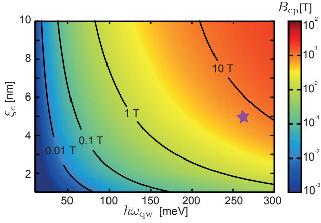
FIG. 10. Log-scale contour-plot of the cavity-protection magnetic field B_{cp} as defined in (37) as a function of the intersubband frequency \omega_{qw} and the disorder correlation length \xi_c . Here, B_{cp} is given in units of Tesla, \hbar\omega_{qw} is given in meV, and \xi_c in nm. The disorder amplitude is kept constant to \xi_0 = 0.3 nm. The effective Bohr magneton corresponding to the effective mass of electrons in GaAs is used, \mu_B^* \approx 0.86 meV / T. The purple star indicates the position of the setup inspired by [17] described in the text.
