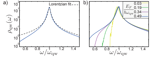
FIG. 3. a) Optical density \rho_{\text{qw}}(\omega) (blue solid line) and Lorentzian fit (black dashed line). b) Optical density \rho_{\text{qw}}(\omega) calculated for increasing values of the Fermi energy E_F . Disorder parameters: \eta_{\text{dis}} \approx 0.06 , \xi_c/l_{\text{qw}} = \sqrt{2} . In a) the Fermi energy is fixed to E_F/\hbar\omega_{\text{qw}} \approx 0.6 , while in b) a range of values is used as indicated in the legend.
