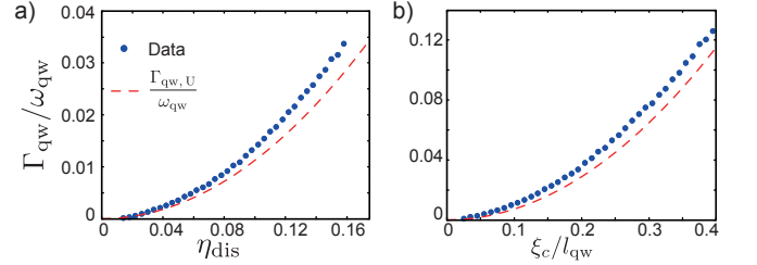
FIG. 4. a) Plot of the FWHM \Gamma_{\text{qw}} of the ISB optical density \rho_{\text{qw}} as a function of the disorder strength \eta_{\text{dis}} (blue solid dots). b) Plot of \Gamma_{\text{qw}} as a function of the disorder correlation strength \xi_c . Disorder parameters: \xi_c/l_{\text{qw}} = 0.5 (in panel a), \eta_{\text{dis}} = 0.4 (in panel b). Fermi energy E_F/\hbar\omega_{\text{qw}} \approx 0.5 . In both panels, the red dashed line is the Unuma-linewidth given by Eq. (23). To numerically implement Eq.(15) we used a finite-width delta function, with small linewidth \gamma_\delta/\omega_{\text{qw}} \approx 0.002 , which is then subtracted from the numerical data.
