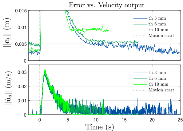
Fig. 4: Target error and computed velocity output during motion.
