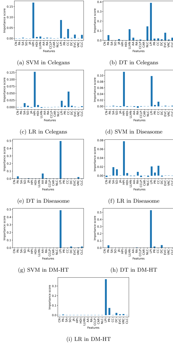
Fig. 3: Feature importance in different datasets by different supervised methods: (a)-(c) in Celegans, (d)-(f) in Disease, (g)-(i) in DM-HT
