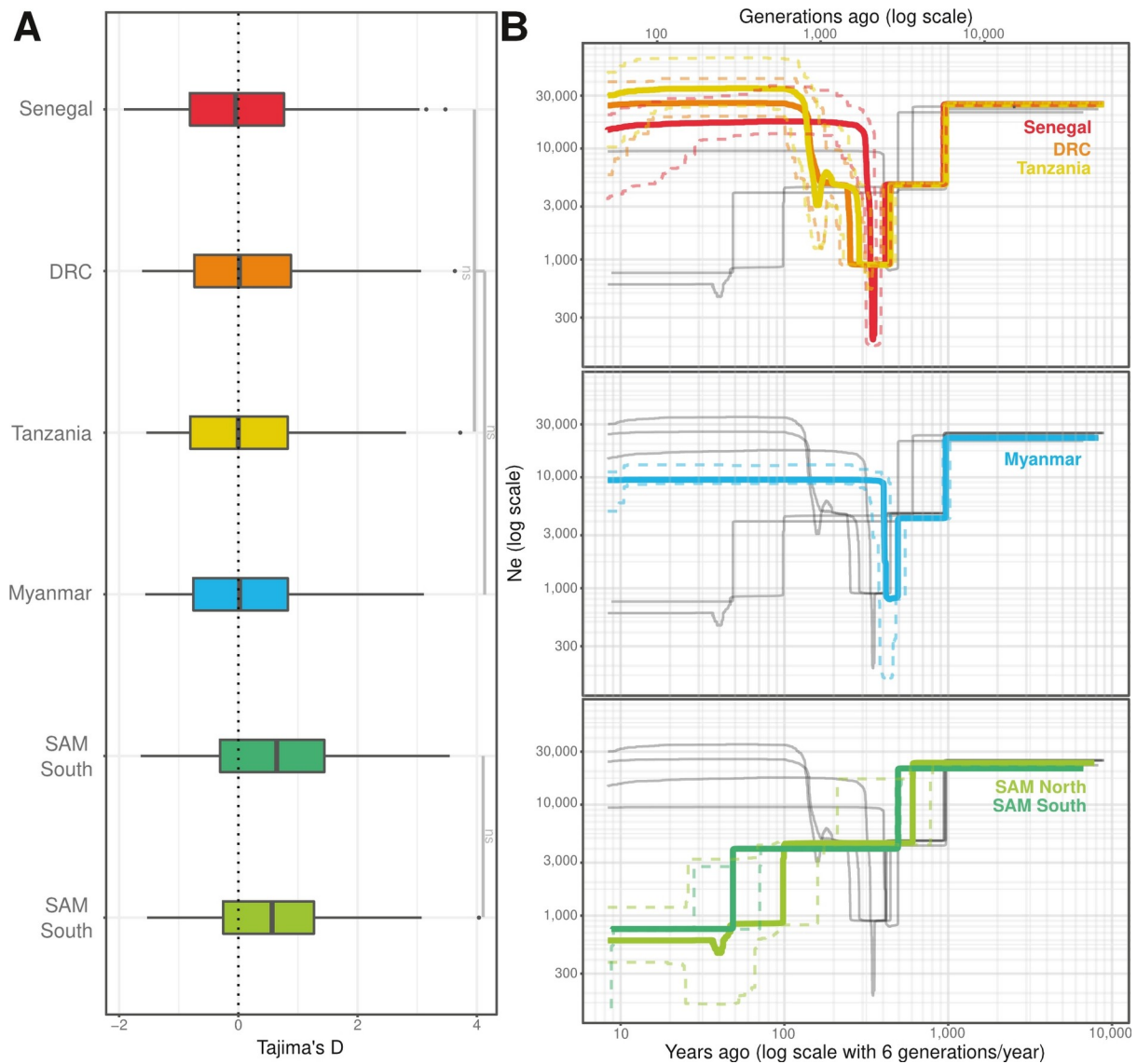
Figure 3: Demographic history of P. falciparum in South America, compared with African and Asian populations. A. Comparison of the Tajima's D values of the two American genetic clusters, three African populations (Senegal, Tanzania, and DRC), and one Asian country (Myanmar). B. Effective population size inferred from Stairway plot 2 for the two American clusters, three African populations (Senegal, Tanzania, and DRC), and one Asian country (Myanmar). The solid lines correspond to the median and the dashed lines represent the 95% confidence interval. Gray lines represents the other populations. Note that the axes are in the \log_{10} scale. DRC: Democratic Republic of Congo.
