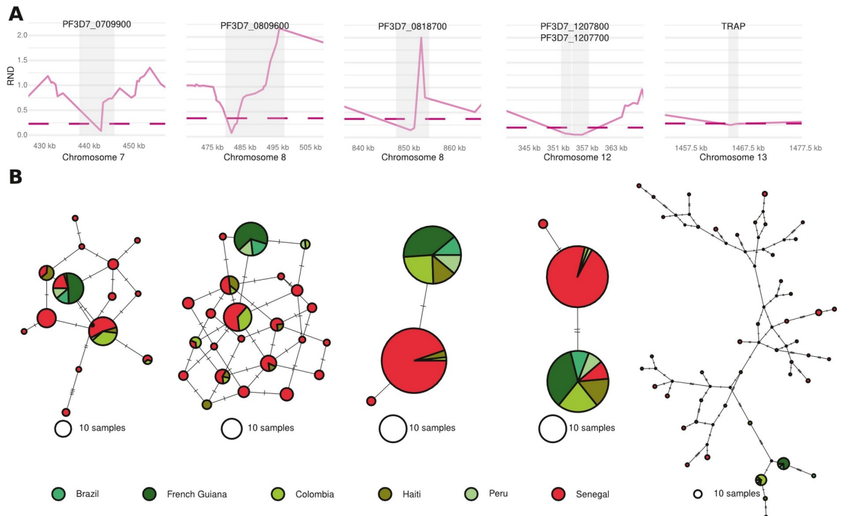
Figure 5: Candidate genes for convergent evolution or introgression between American clusters. A. Relative Node Depth (RND) values between SAM North (Haiti - Colombia) and SAM South (Brazil - French Guiana) for five regions. The region in gray represents the gene (gene name on top). The dotted line marks the 5% threshold of the lowest values on the chromosome. B. Median-Joining haplotype networks of the regions with the lowest RND values between American clusters. TRAP: thrombospondin-related adhesive protein.
