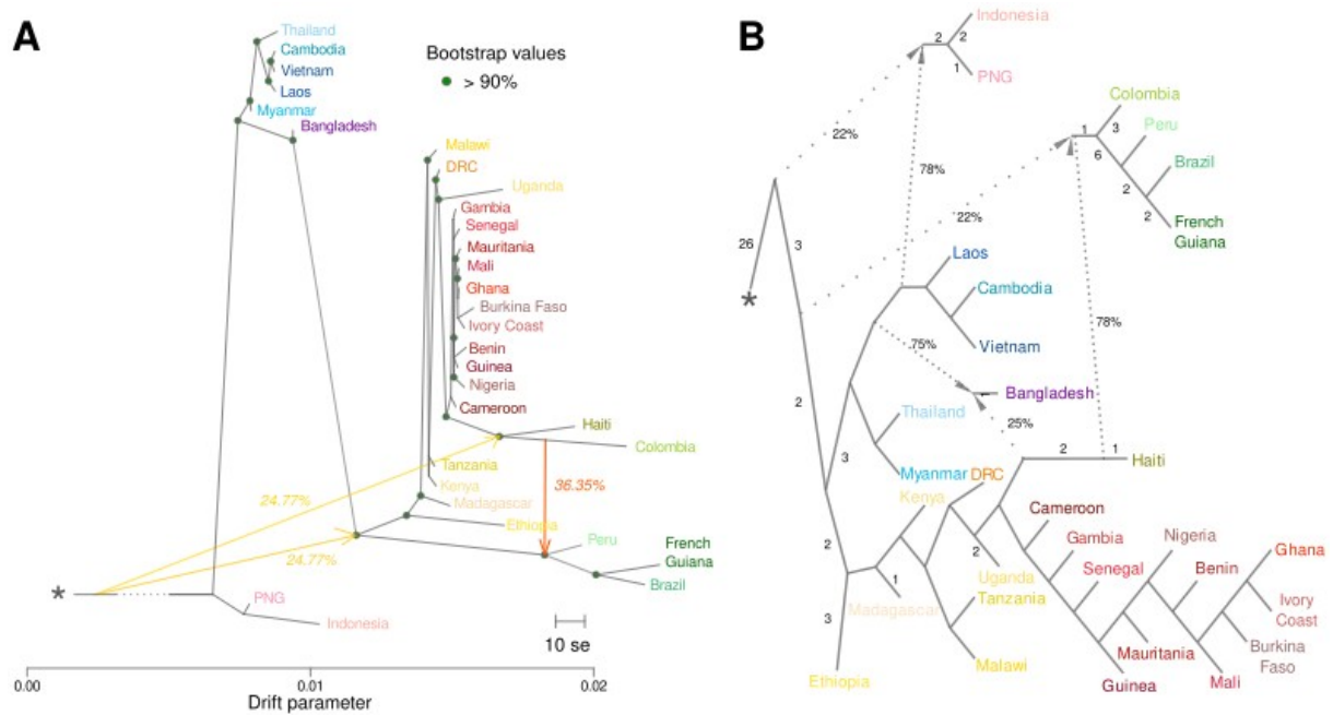
Figure 2: Relationships and admixture proportions between P. falciparum populations. A. TreeMix tree of P. falciparum populations with three migration edges (arrows), rooted with P. praefalciparum . Filled circles represent the bootstrap values supported by more than 90%. The scale bar shows ten times the mean standard error (se) of the entries in the sample covariance matrix. Arrows show the migration edges between tree branches. The migration weight is indicated by the yellow (low) to red (high) color gradient and the estimated value is shown as a percentage on the migration edge. B. Admixture graph of P. falciparum populations, with three admixture events, rooted with P. praefalciparum . Admixture events (and the estimated percentages) are shown with dash arrows that connect the admixed population with the two source population branches. The number on each branch represents the branch length that indicates the amount of drift accumulated along that branch (in f -statistic units, multiplied by 1,000 and rounded to the nearest integer). Branches without a number are branches with a drift score = 0. PNG: Papua New Guinea, DRC: Democratic Republic of Congo. The asterisk represents the P. praefalciparum outgroup.
