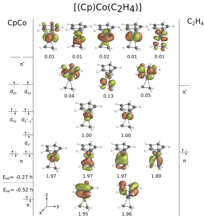
Fig. 3 CASSCF natural orbital diagram of [(\text{Cp})\text{Co}(\text{C}_2\text{H}_4)] (triplet state) with partial occupation number, CAS(14,16).
