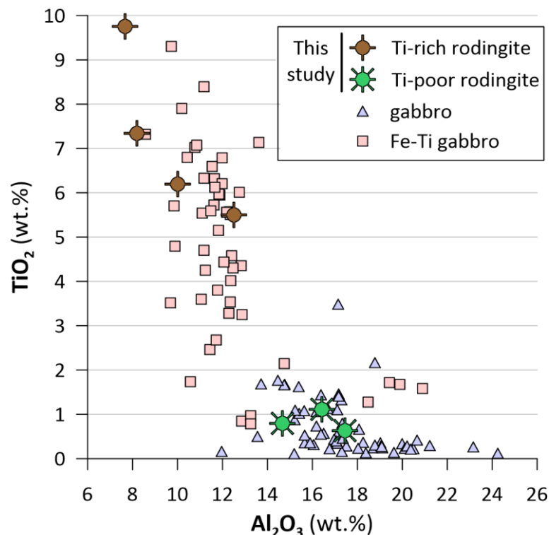
Figure 13 TiO 2 versus Al 2 O 3 diagram comparing the whole rock composition of studied rodingites with proposed types of gabbroic protolith. Data for common magnesian (meta)gabbro (Schwartz et al. 2000; Montanini et al. 2006; Miller et al. 2007; Bucher and Grapes 2009; Bucher and Stober 2021) and Fe-Ti (meta)gabbro (Liou et al. 1998; Schwartz et al. 2000; Montanini et al. 2006; McCarthy and Müntener 2019; Starr et al. 2020) are from ophiolite occurrences from the Alpine-Apennine orogenic belt. All data were recalculated on anhydrous basis in wt.%. Assuming restricted mobility of Ti and Al during metasomatic and/or metamorphic process, we infer a common gabbro as protolith for the Ti-poor samples and a Fe-Ti gabbro for the Ti-rich rodingites from Bôrček.
