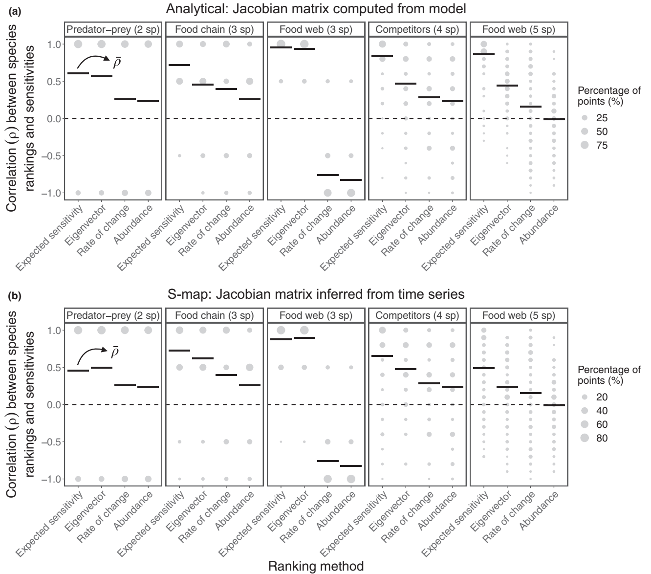
FIGURE 3 Expected sensitivity and eigenvector approaches allow us to accurately rank species sensitivities to perturbations under several population dynamics models. (a) Rank correlation ( \rho ) between species sensitivities to perturbations ( \langle s_i \rangle ) and four different approaches (expected sensitivity, \mathbb{E}(s_i) ; eigenvector, |\mathbf{v}_{1i}| ; rate of change, \Delta N_i(t) ; and abundance, -N_i(t) ). Note that the Jacobian matrix and, therefore, \mathbb{E}(s_i) and |\mathbf{v}_{1i}| are computed analytically from the model. Each panel shows the percentage of points with a given \rho value (size of grey points) and the average of these values across time ( \bar{\rho} , black horizontal lines) for a synthetic time series generated from the corresponding population dynamics model. (b) Same as (a) but with the Jacobian matrix and, therefore, \mathbb{E}(s_i) and |\mathbf{v}_{1i}| inferred with the S-map using only past time-series data. In (a), the expected sensitivity approach shows a higher \bar{\rho} than the other three ranking approaches under all models. In (b), the expected sensitivity approach outperforms the eigenvector approach for three out of five models.
