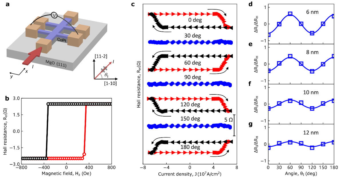
Figure 2 | Field-free magnetization switching in \text{Co}_{30}\text{Pt}_{70} single layers on \text{MgO} (111) substrate. a , Schematic of the \text{Co}_{30}\text{Pt}_{70} Hall bar device for electrical transport measurement. b , Anomalous Hall effect of the 6 nm \text{Co}_{30}\text{Pt}_{70} sample. c , Current-induced field-free magnetization switching in \text{Co}_{30}\text{Pt}_{70} for Hall bars with different \theta_1 . The loops are manually shifted for better visualization. d-f , \theta_1 dependence of \Delta R_l/\Delta R_H for \text{Co}_{30}\text{Pt}_{70} devices with different thicknesses (6, 8, 10 and 12 nm).
