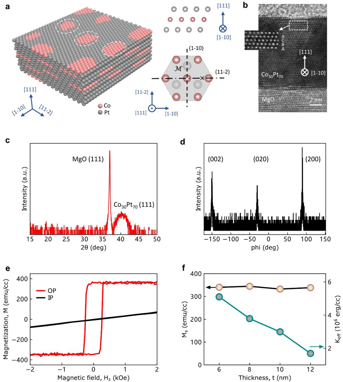
Figure 1| Structural and magnetic properties of \text{Co}_{30}\text{Pt}_{70} thin film. a , left, the schematic illustration of \text{Co}_{30}\text{Pt}_{70} with randomly located Co platelets (see white circles); right top, the side view of the Co platelet/Pt structure; right bottom, the mirror symmetry analysis of Co platelet/Pt, where [1-10] is defined as the low-symmetry axis and [11-2] as the high-symmetry axis, respectively. b , High-resolution transmission electron microscopy (HR-TEM) image of \text{Co}_{30}\text{Pt}_{70} with [1-10] pointing inward. The area within the dotted rectangle was amplified to present the stacking sequence (ABCABC...) of \text{Co}_{30}\text{Pt}_{70} . c , High-resolution X-ray diffraction
