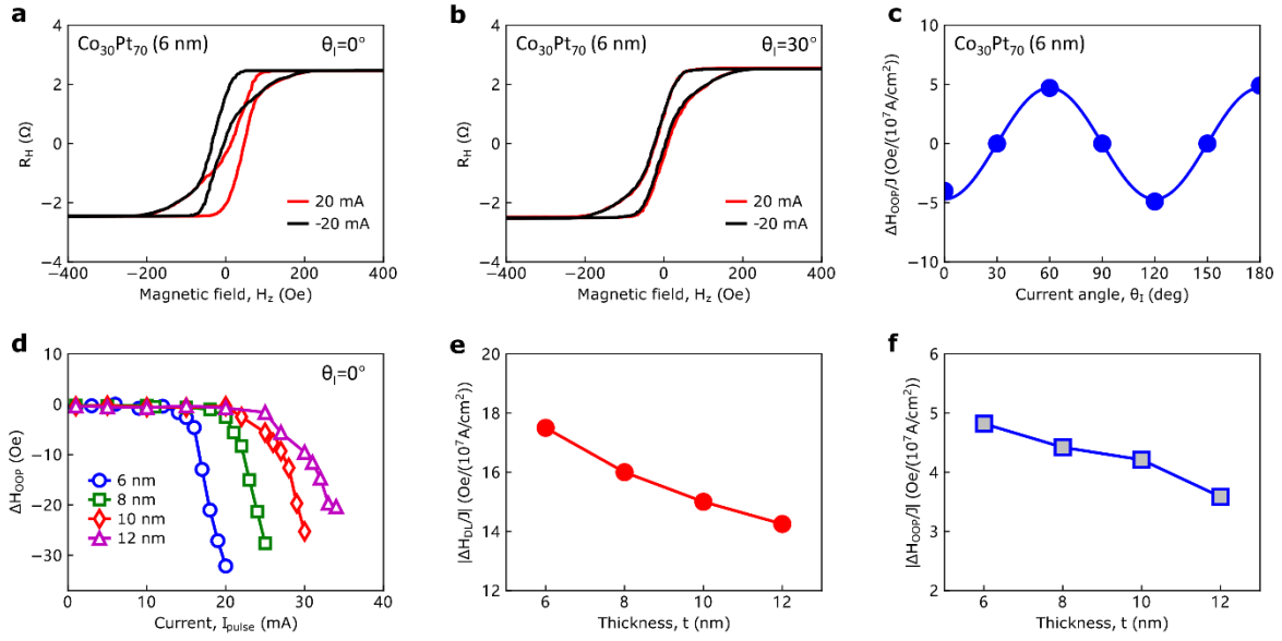
Figure 3| Current-induced out-of-plane and in-plane SOT effective fields. a-b, AHE loops under +20 mA and -20 mA pulsed currents for \theta_1=0 deg (a) and 30 deg (b). c, Current angle dependence of the out-of-plane effective field efficiency ( \Delta H_{OOP}/J ) in 6 nm \text{Co}_{30}\text{Pt}_{70} . d, Current dependence of \Delta H_{OOP} for various \text{Co}_{30}\text{Pt}_{70} thicknesses. e, f, Thickness dependences of in-plane and out-of-plane SOT effective fields for \theta_1=0 deg, respectively. The \Delta H_{OOP} for the largest measured current in d is used for the calculation in f .
