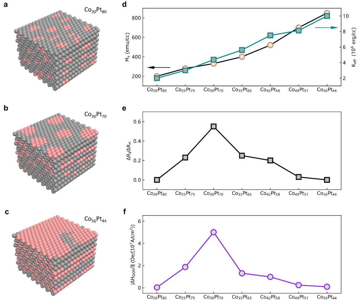
Figure 4| Composition dependence of the OOP effective fields and switching behavior in \text{Co}_x\text{Pt}_{100-x} single layers. a-c , Tentative structures of \text{Co}_{20}\text{Pt}_{80} , \text{Co}_{30}\text{Pt}_{70} and \text{Co}_{56}\text{Pt}_{44} , which correspond to the lowest, optimal and highest Co compositions in our experiments, respectively. A large disordered background was omitted in these structures for easier analysis. Since the Co platelets are mainly distributed near the substrate, the top side of the structure in b is adjacent to the substrate. d , Composition dependence of M_s and K_{\text{eff}} in \text{Co}_x\text{Pt}_{100-x} single layers. e , Composition dependence of \Delta R_l/\Delta R_H in \text{Co}_x\text{Pt}_{100-x} single layers. f , Composition dependence of \Delta H_{\text{OOP}}/J in \text{Co}_x\text{Pt}_{100-x} single layers.
