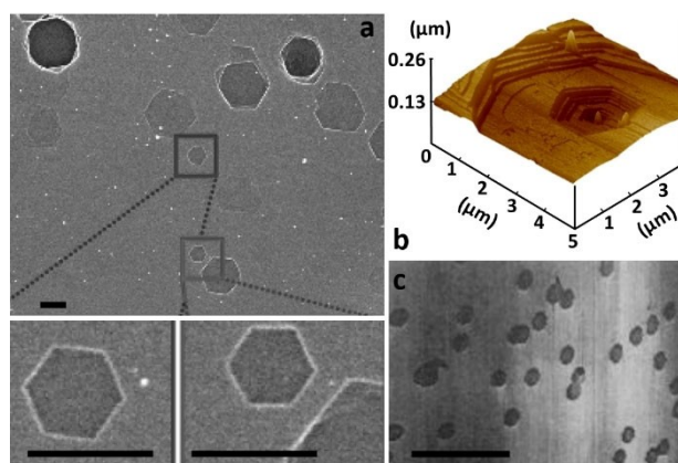
Figure 5. SEM (a), AFM (b) and STM (c) images of HOPG surfaces after partial oxidation. Value for the scale bar (a and c) is 1 \mu\text{m} . Carbon combustion occurs not randomly on the carbon basal plane but is occurring on specific sites (also called active surface sites). Typically, the reaction occurs in proximity to the initial active sites due to progressive formation of reactive sites in the course of the carbon combustion (see also chapter 6 for a more detailed discussion). Adapted with permission from Ref. [20, 23, 24]. Copyright 2022, Wiley-VCH.
