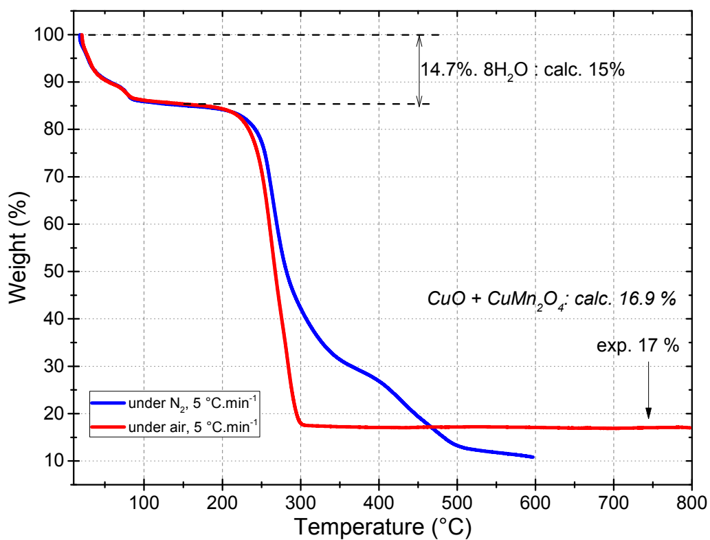
Figure S4. TGA of 1 performed under air or N 2 .
