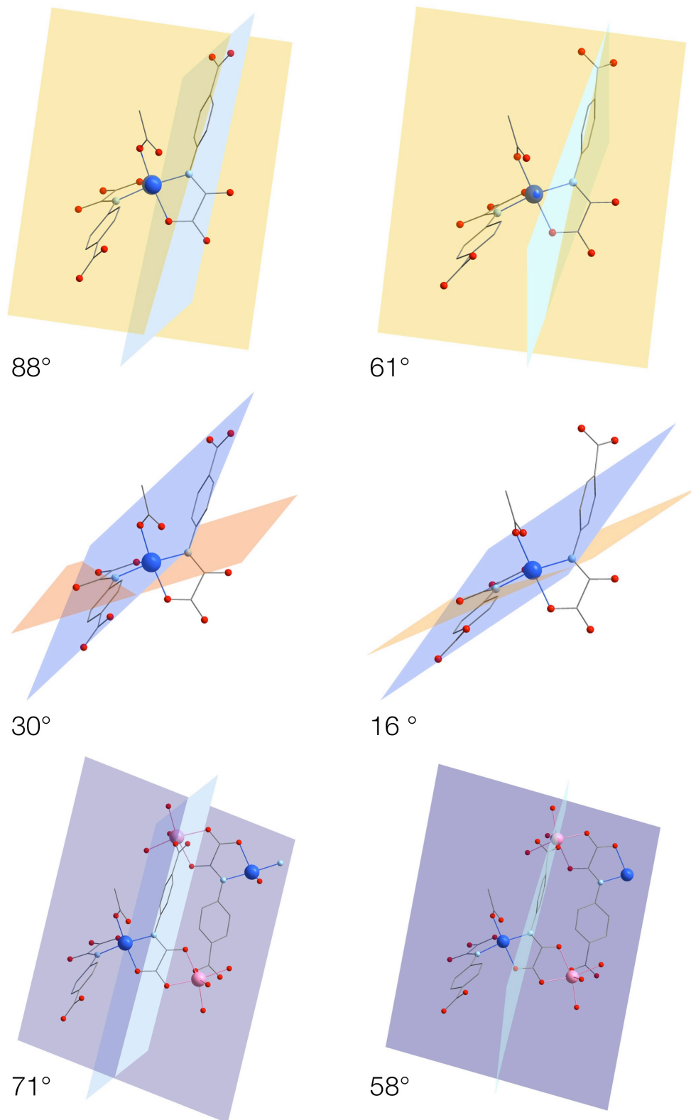
Figure S7. Representation and values of the dihedral angles in 1 and 1b. Phenyl ring/oxamate plane in the [\text{Cu}(\text{paba})_2(\text{OAc})]^{5-} building complex and phenyl ring/phenyl ring along the brick-wall structure rung \{\text{Cu}_2\text{Mn}_2(\text{paba})_2\} .
