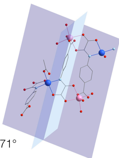
Figure S7. Representation and values of the dihedral angles in 1 and 1b. Phenyl ring/oxamate plane in the [\text{Cu}(\text{paba})_2(\text{OAc})]^{5-} building complex and phenyl ring/phenyl ring along the brick-wall structure rung \{\text{Cu}_2\text{Mn}_2(\text{paba})_2\} .
