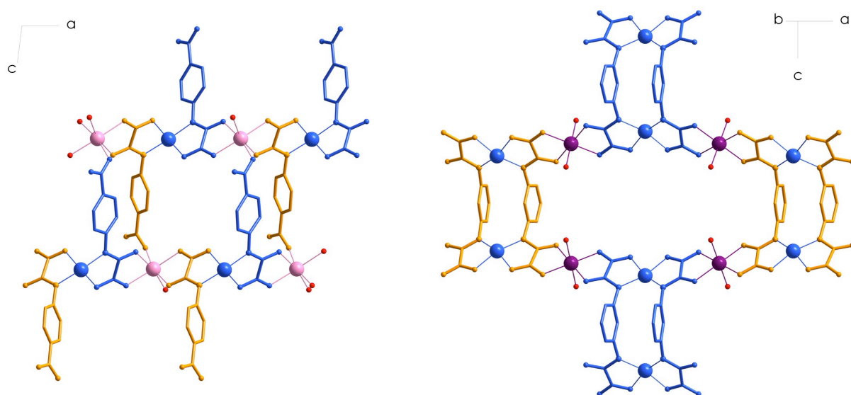
Figure 3. Comparison of the brick-wall arrangements in 1 (left) and in [\text{Co}_2\text{Cu}_2(\text{mpba})_2(\text{H}_2\text{O})_6] (right). 42 H atoms, (\text{TMA})^+ counter-cations, acetate groups and solvent molecules are omitted for clarity.
