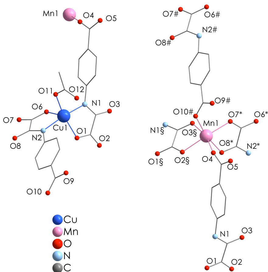
Figure 1. Representation of the coordination environments of the Cu(II) and Mn(II) ions together with selected atom labels (#: x, y, -1+z ; *: 1/2+x, 1/2-y, -1/2+z ; §: -1/2+x, 1/2-y, -1/2+z ). H atoms are omitted for clarity.
