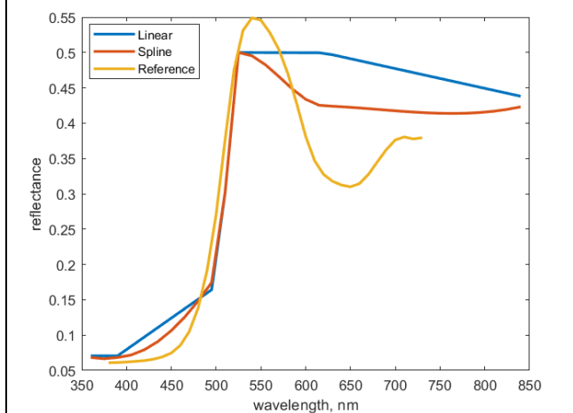
Patch 11 Yellow green reference and interpolated (Linear & Spline)
