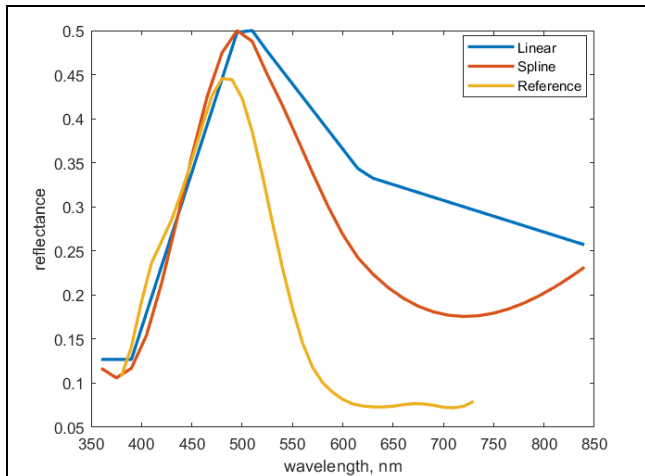
Patch 18 Cyan reference and interpolated (Linear & Spline)
