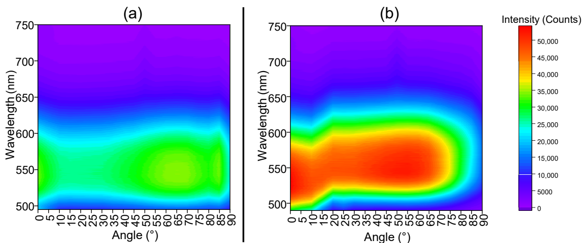
Figure 6. Luminescence maps corresponding to the emission spectra under a 458 nm excitation detected at different angle positions for (a) non-structured YAG:Ce and (b) nanostructured ZnO NWs/YAG:Ce coatings. The color code represents the emission intensity.
