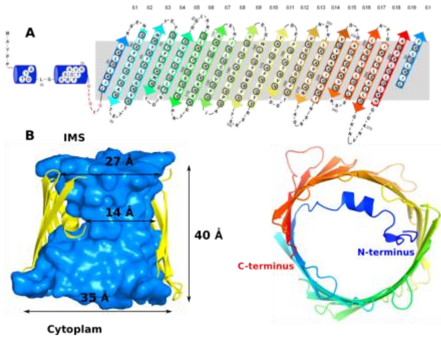
Fig. 9.2 Structural overview of mVDAC1. (A) Topology of the primary sequence. (B) Cartoon representation of mVDAC1 based of PDB file 3EMN. The left panel is the view from the membrane, and the right panel is the view the top down view from the inter-membrane space. Adapted from (Ujwal et al., 2008).
