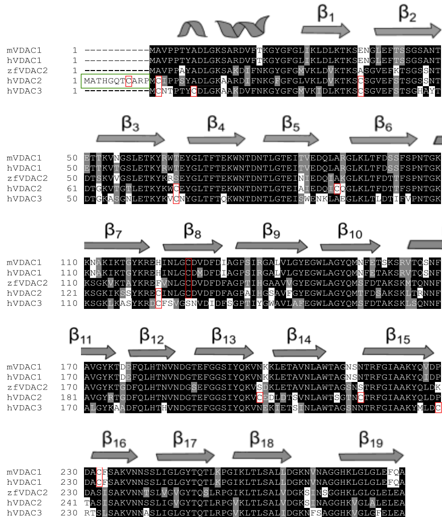
Fig. 9.1 Comparison of VDAC isoforms. Sequence alignment of several VDAC isoforms: mVDAC1 (Q60932), hVDAC1 (P217796), zfVDAC2 (Q8AWD0), hVDAC2 (P45880), and hVDAC3 (Q9Y277). The second structure elements are represented on top of the sequence for reference. The cysteine residues are shown in red boxes, and the N-terminal extension of 11 amino acids of hVDAC2 are shown in green.
