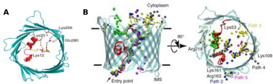
Fig. 9.6. ATP permeation through VDAC. (A) Cartoon representation of mVDAC1 in complex with ATP (PDB code 4C69). (B) Representation of the five primary pathways of ATP permeation, dots represent the \gamma -Phosphate of ATP. ATP permeates the pore via several distinct pathways each lined with basic residues that interact electrostatically with the phosphate group. The arrow indicates the common entry point. Reprinted from (Choudhary et al., 2014).
