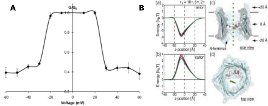
Fig. 9.5. Conduction properties of VDAC. (A) Conductance profile of mVDAC1 shows a bell-shaped curve with high conductance near 0 mV, but reduced conductance at values below -30 mV and above +30 mV (Ujwal et al., 2008). (B) The electrostatic energy profile for anions (a) and cations (b) to move through the channel. The ion pathways traversed in panels a and b are shown from the side view from the membrane (c) and from the cytoplasm. The negative energy in panel a indicates that anions are favored in the pore. Reprinted from (Choudhary et al., 2010) with permission from Elsevier.
