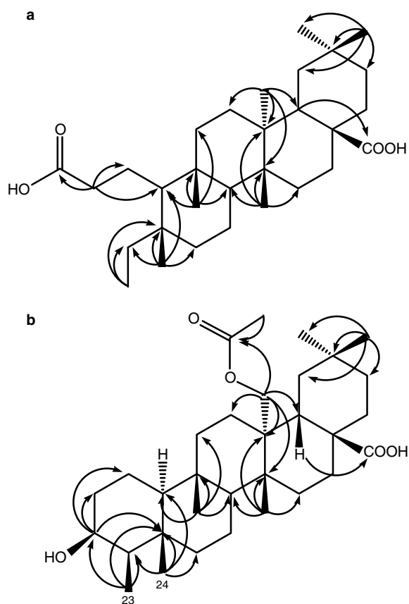
Scheme 2. Partial HMBC correlations (H → C) for (a) 3,4-secofriedelan-3,28-dioic acid ( 1 ) and (b) 27-Hydroxyacetate canophylllic acid ( 2 ).
