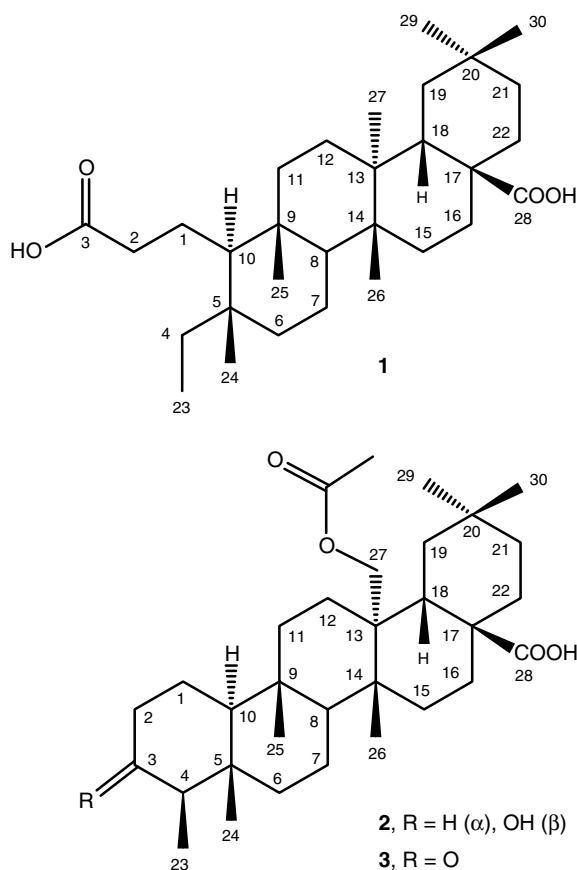
Scheme 1. Structures of triterpenes 1–3 .
