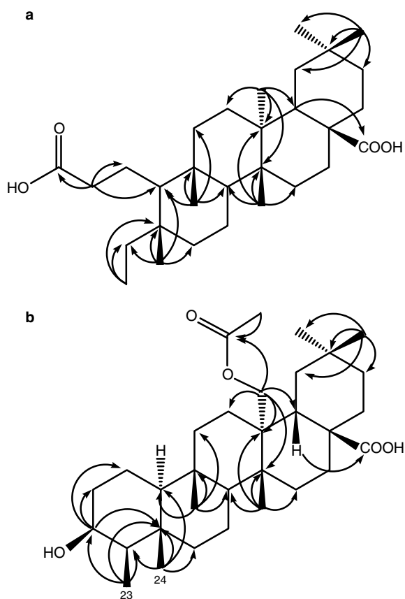
Scheme 2. Partial HMBC correlations (H \rightarrow C) for (a) 3,4-secofriedelan-3,28-dioic acid ( 1 ) and (b) 27-Hydroxyacetate canophylllic acid ( 2 ).
