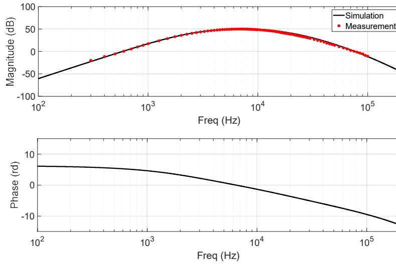
Fig. 8 – MAX274ACN analogic filter Bode plots, comparison measurement/simulation.
