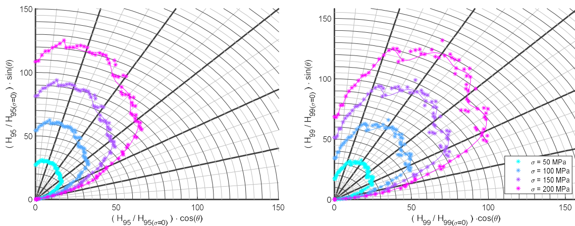
Fig. 13 – FeCo alloy : Evolution of the predicted normalized (a) H_{95} and (b) H_{99} indicators under 50, 100, 150 and 200 MPa tensile stress applied along RD as a function of the orientation of the MBN sensor from RD to TD. The dots show the result of the calculation while the lines are just guide for the eyes.
