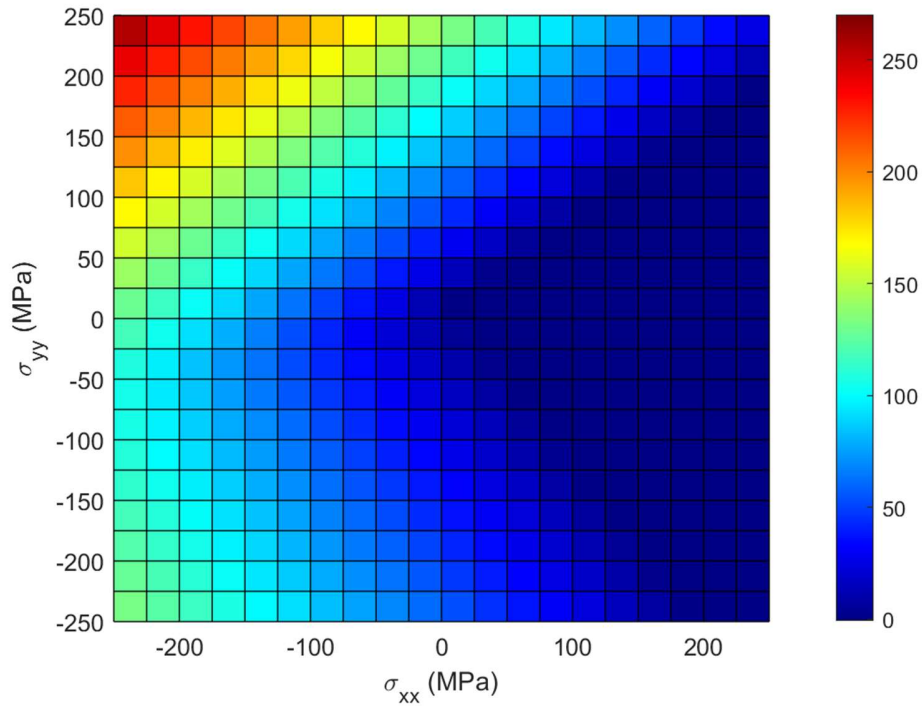
Fig. 14 – FeCo alloy: Evolution of the predicted normalized H_{95} under biaxial stress states. The MBN sensor is positioned along \sigma_{xx} (RD).
