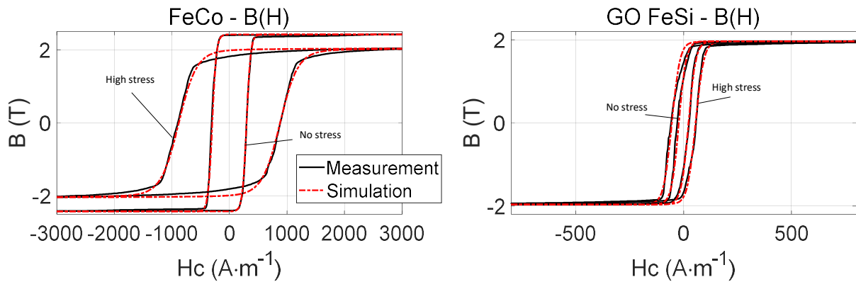
Fig. 9 Comparisons simulations/measurements for the B(H) hysteresis cycles.
