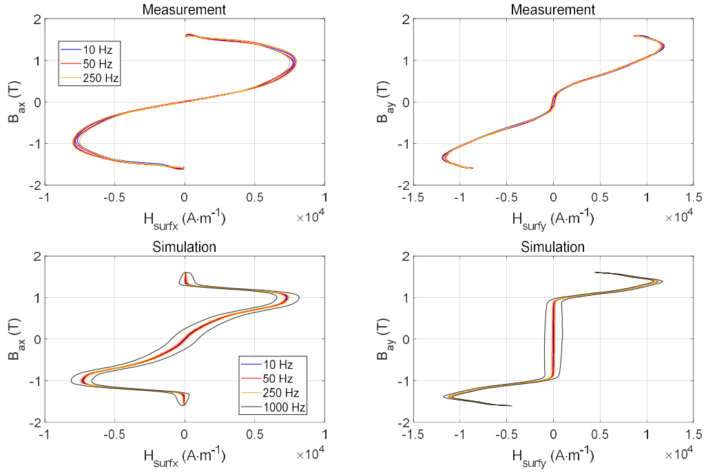
Fig. 11. Plots of B_{ax} versus H_{surf_x} in the rolling direction (RD) and B_{ay} versus H_{surf_y} in the transverse direction (TD) obtained experimentally for FeSi 3 wt% laminated GO electrical steel [49] and those obtained from the optimized vector DF model, which include results obtained at f = 1000 Hz for illustration purposes.
