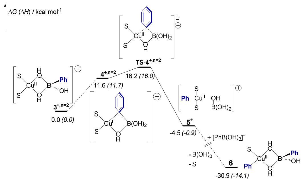
Figure 5. Reaction profile of the Cu-to-B transmetalation in the heterobimetallic cationic intermediate [(S)_2Cu(\mu-OH)_2B(Ph)(OH)]^+ ( 3^{+,n=2} ) ( S = \text{MeOH} ) computed at the DFT level. \Delta G ( \Delta H ) are given in \text{kcal mol}^{-1} . See the Figures S14-16 for alternative pathways.
