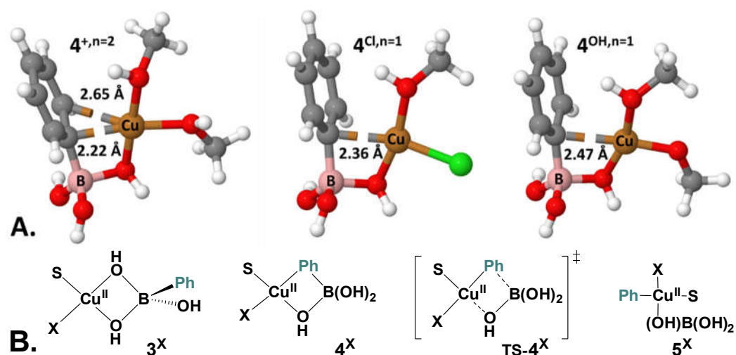
Figure 6. A. 3D structures of optimized intermediates 4^{X,n} (X = +, Cl or MeO, n = 1 or 2). H in white, C in grey, O in red, B in pink, Cu in orange and Cl in green. B. Structures of intermediates and transition states involved in the B-to-Cu transmetalation (see Table 1 for the associated energies). See Figures S15-16 for alternative solvation states.
