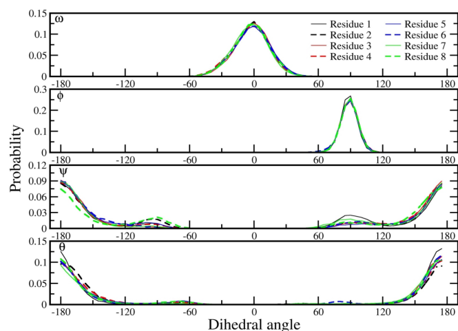
Figure 4. Probability distribution of dihedral angles from 50 ns simulation of (+)_8 \beta -NtBu octapeptoid.
