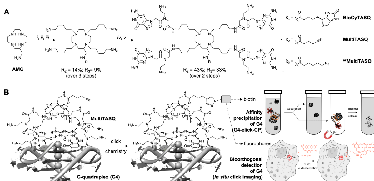
Figure 1. A. Chemical structure and synthesis of BioCyTASQ, MultiTASQ and az MultiTASQ; i : R-CO 2 H, TSTU, DIPEA, DMF; ii : MsO-(CH 2 ) 5 -NHBoc, K 2 CO 3 , CH 3 CN; iii : TFA; iv : Boc- PNA G-OH, HBTU, DIPEA, DMF; v : TFA. B. Schematic representation of the G-quartet/G-quartet interaction between the TASQ and a DNA/RNA G4, and of the click chemistry-based investigations made possible with MultiTASQs, i.e. , G4 isolation by affinity capture (clicked biotin) and optical imaging (clicked fluorophore).
