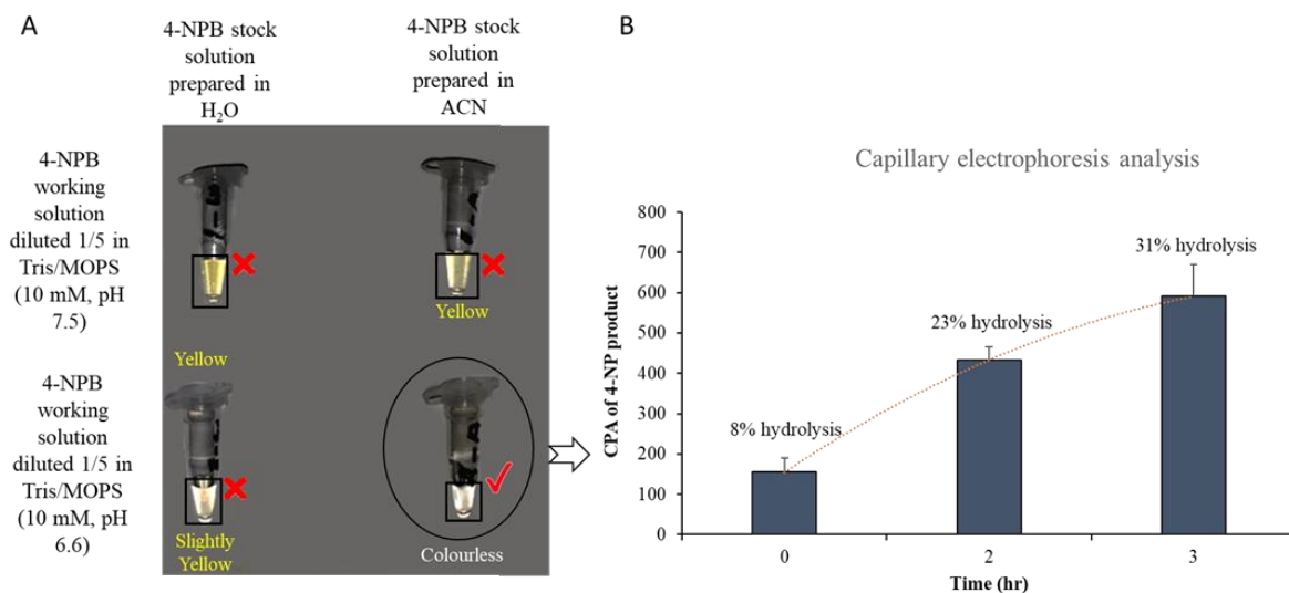
Figure 5. Visual spontaneous hydrolysis of 4-NPB in the absence of PL. A) The yellow color represents the release of 4-NP as a result of spontaneous 4-NPB hydrolysis. The substrate was prepared at a stock concentration of 5 mM in either water (left) or ACN (right). 10 \mu L of 5 mM 4-NPB was then mixed with 40 \mu L of 10 mM Tris/ 40 mM MOPS (Ionic strength= 10 mM, pH 7.5 (top row) or pH 6.6 (bottom row)) to have a final substrate concentration of 1 mM and a final volume of 50 \mu L. The mixtures were incubated at 37 ^{\circ} C for 5 min and then at 95 ^{\circ} C for another 5 min before the color of each tube was observed. B) CE injection at different time points of 4-NPB solution prepared in ACN and diluted in Tris/MOPS (10 mM, pH 6.6) to estimate time dependent spontaneous hydrolysis.
