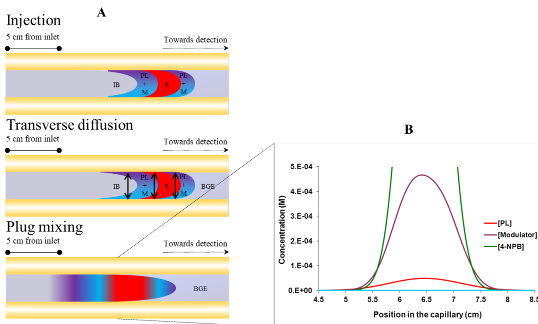
Figure 2. Schematic representation of the different steps of the online enzymatic reaction A ). Injection of the different reactants sequentially into the capillary filled with the BGE as follows; 8 mg mL -1 PL + 1 mg mL -1 of the
