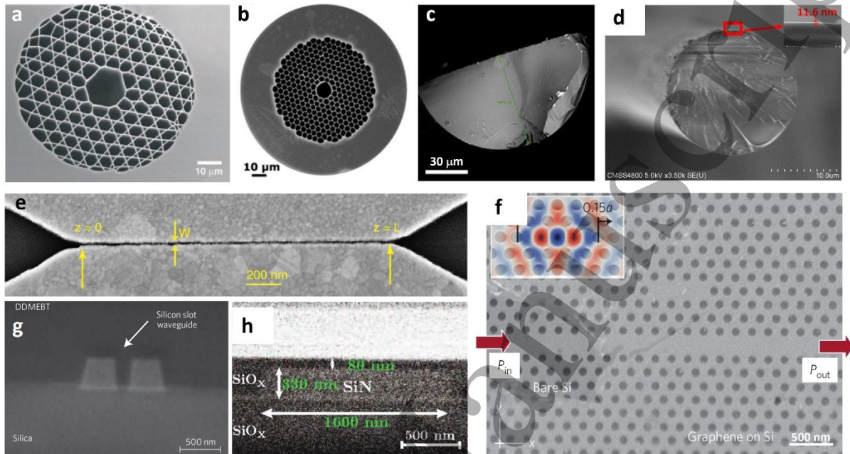
Fig. 8. SEM images of NLO hybrid fibers and hybrid on-chip waveguides. The labels of the sub-figures correspond to the labels given in Tables 8A and 8B. Panels a and e are reprinted with permission from [Benabid2002, Nielsen2017], AAAS. Panels b, f, and g are reprinted with permission from [Yang2020, Gu2012, Koos2009], Springer Nature. Panels c and h are reprinted with permission from [An2020, Alexander2017], ACS. Panel d is reprinted with permission from [Wang2018], CLP Publishing.
