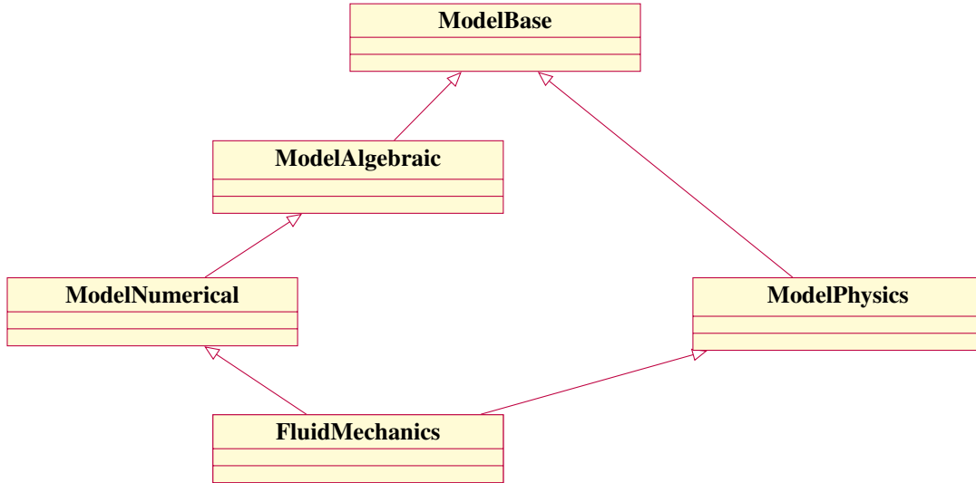
Figure 7: UML diagram of the FluidMechanics class.
