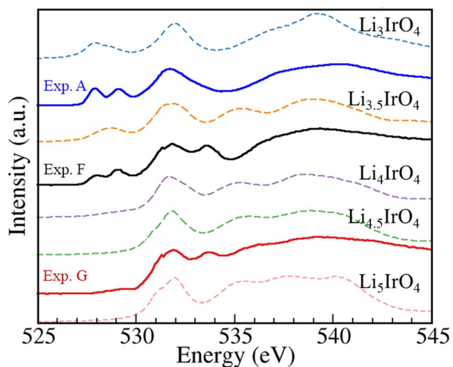
Figure 4. Simulated O K-edge XAS spectra of different electrochemical states and the corresponding experimental results. The XAS projected on the O_{\text{up}} and O_{\text{down}} absorbing species are shown in Fig. S4. The peak at \sim 533.7 eV in the experimental data is ascribed to the presence of \text{Li}_2\text{CO}_3 impurity.
