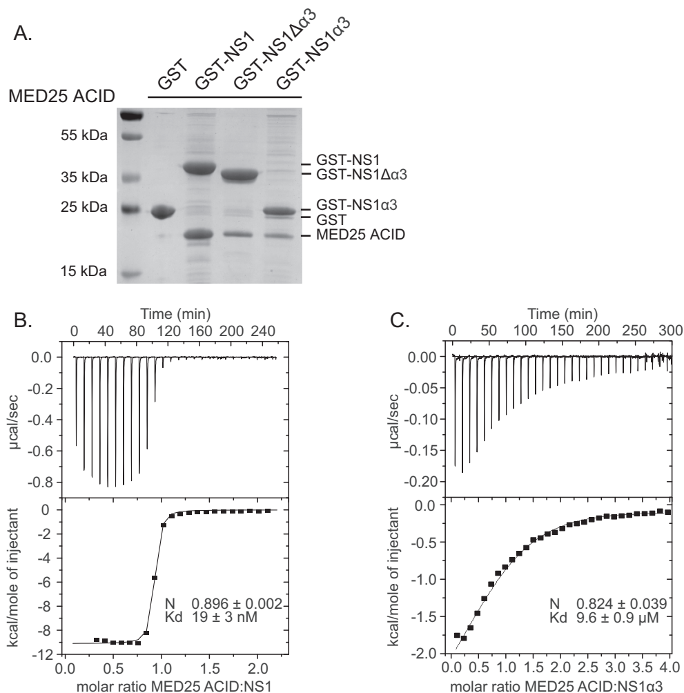
Figure 3. NS1-MED25 ACID interaction by GST pull-down assay and by isothermal titration calorimetry. (A) MED25 ACID was co-expressed together with GST, GST-NS1, GST-NS1 \Delta\alpha 3, or GST-NS1 \alpha 3 in E. coli BL21(DE3) bacteria. Bacteria lysates were clarified and the soluble protein complexes were purified on glutathione-Sepharose beads. After extensive washing the binding of MED25 ACID to GST, GST-NS1, GST-NS1 \Delta\alpha 3 and GST-NS1 \alpha 3 was analysed by SDS-PAGE and Coomassie blue staining. (B) and (C) Binding of MED25 ACID to NS1 protein and to NS1 \alpha 3 peptide was measured by isothermal titration calorimetry. 300 \mu M MED25 ACID was titrated into 20 \mu M NS1, and 420 \mu M MED25 ACID was titrated into 20 \mu M NS1 \alpha 3, with 8 \mu L injection volumes. The upper panel shows the raw heat release data after baseline correction. The lower panel shows the integrated ITC data (filled squares) fitted with a one set of sites binding model (straight line). Dissociation constants ( K_d ) and stoichiometric ratios (N) obtained from the fit are indicated on the lower panel.
