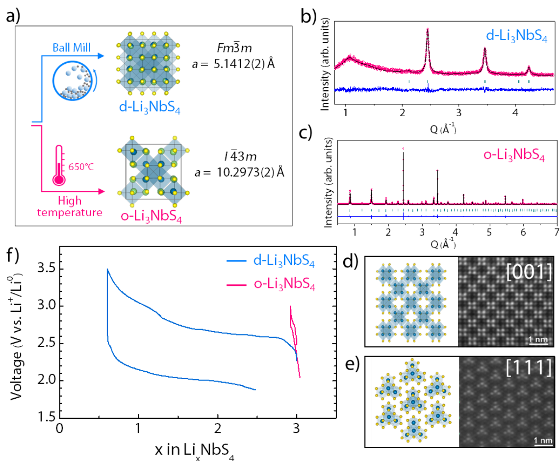
Figure 1: (a) Structures of d-Li 3 NbS 4 and o-Li 3 NbS 4 with the corresponding methods of synthesis in the left. (b) X-ray Rietveld refinement of d-Li 3 NbS 4 (resp. o-Li 3 NbS 4 ) at 300 K. (c) X-ray Rietveld refinement of o-Li 3 NbS 4 at 300 K. The wavelength used for synchrotron X-ray is \lambda = 0.4137\text{\AA} . For both (b) and (c) the pink circles, black continuous line, and bottom blue line represent the observed, calculated, and difference patterns, respectively. Vertical green tick bars stand for the Bragg positions. These plots can be found enlarged in the figure S3. (d) and (e) high resolution HAADF-STEM images of o-Li 3 NbS 4 along [001] and [111] directions and the corresponding structure projections. (f) First cycle voltage–composition trace of d-Li 3 NbS 4 (blue) and o-Li 3 NbS 4 (pink) starting with oxidation and cycled at C/20.
